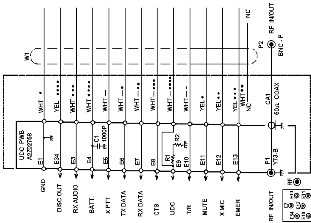
UDC CONNECTOR PIN ASSIGNMENT (FRONT VIEW)
